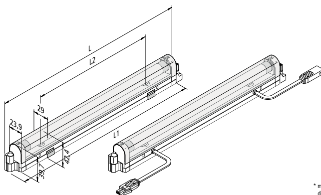
assembly arrangement with admissible clearances
