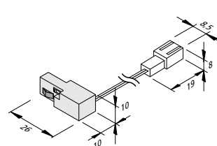
adapter
