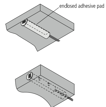
mounting arrangement
