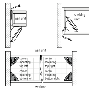
mounting arrangement (examples)
