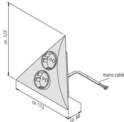
mounting arrangement (examples)
