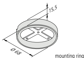
mounting ring
